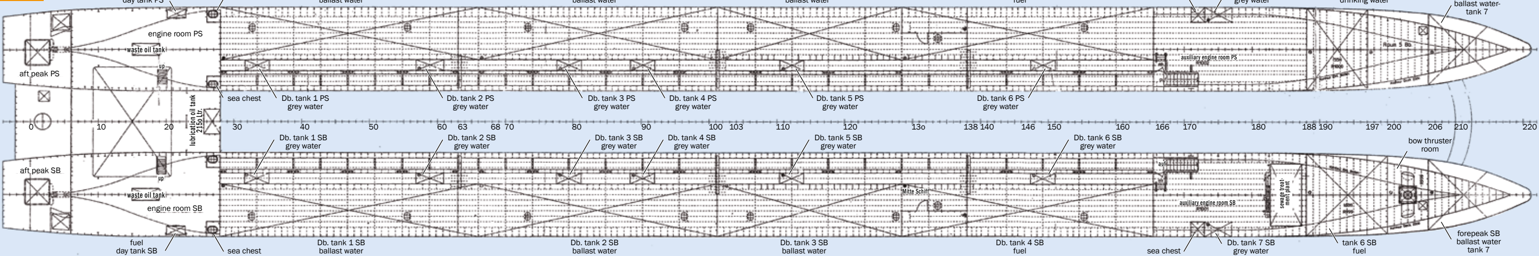
00 | Lower deck
