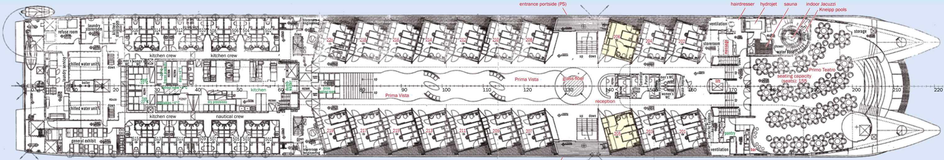
01 | Main deck
